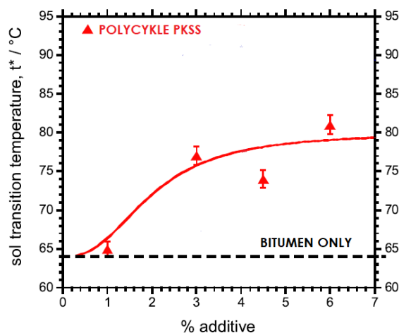
Variation of the transition temperature between elastic and viscous behavior of bitumen modified with POLYCYKLE PKSS
